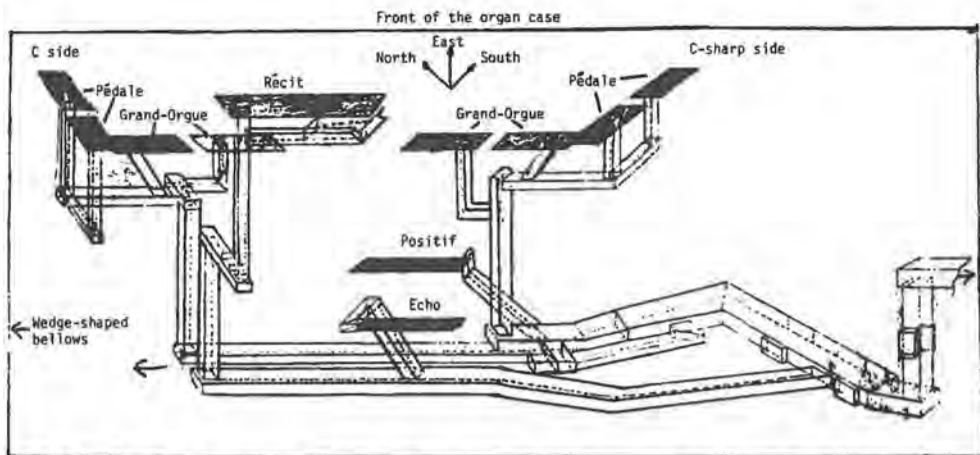
Jean Deloye's design of the wind trunks leading to the various windchests of the Dole organ.
